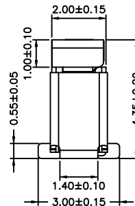
KAPTON TAPE (FOR PICK AND PLACE SYSTEMS)
