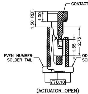
(ACTUATOR OPEN)
